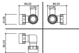
ELBOW FxM 1"
