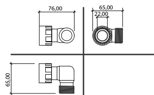
NIPPLE 1"
