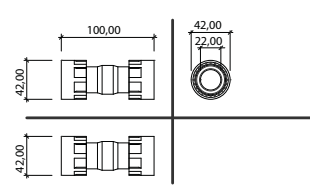
NIPPLE 1" x 3/4"
