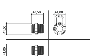
NIPPLE 1"
