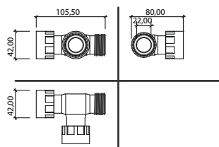
CROSS FxFxFxM 1"
