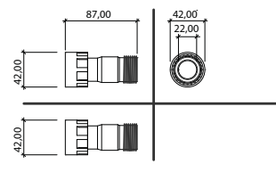
COUPLING FxF 1"
