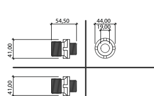
NIPPLE 1" x 3/4"
